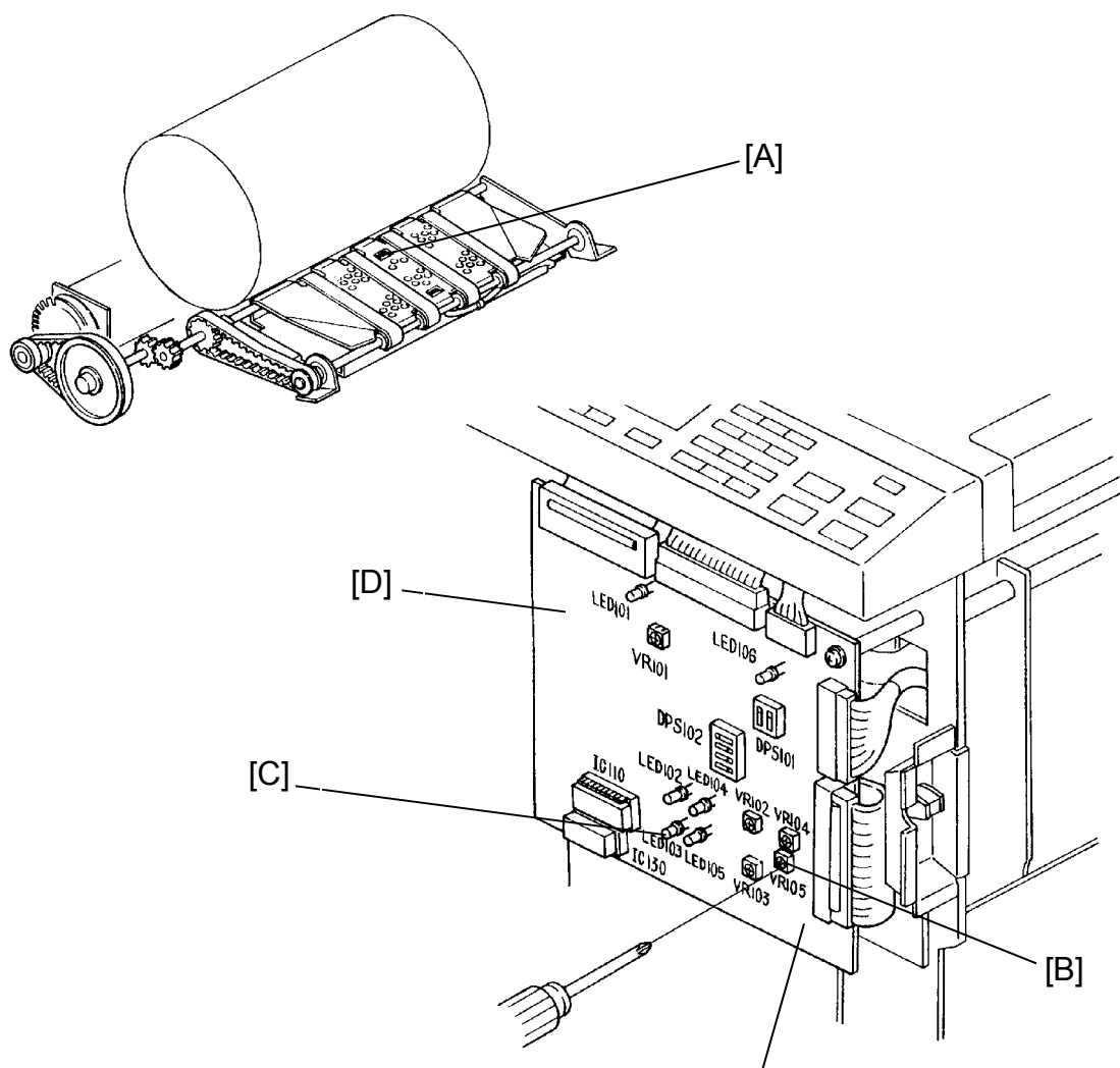
VT2300/VT2500 Main Control Board
